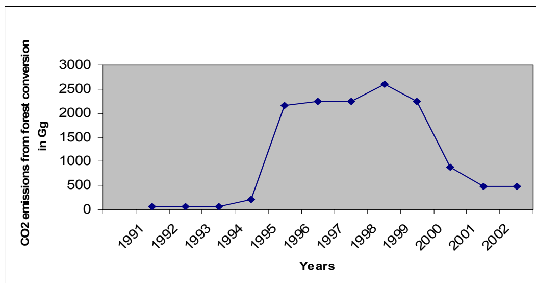
Diag 33: CO 2 emissions from forests conversion
