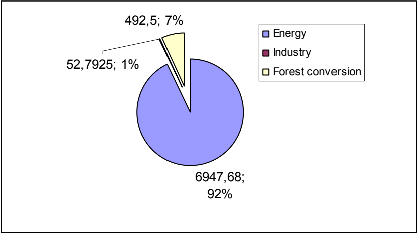
Diag 40: Total GHG emissions in Gg in 2002
